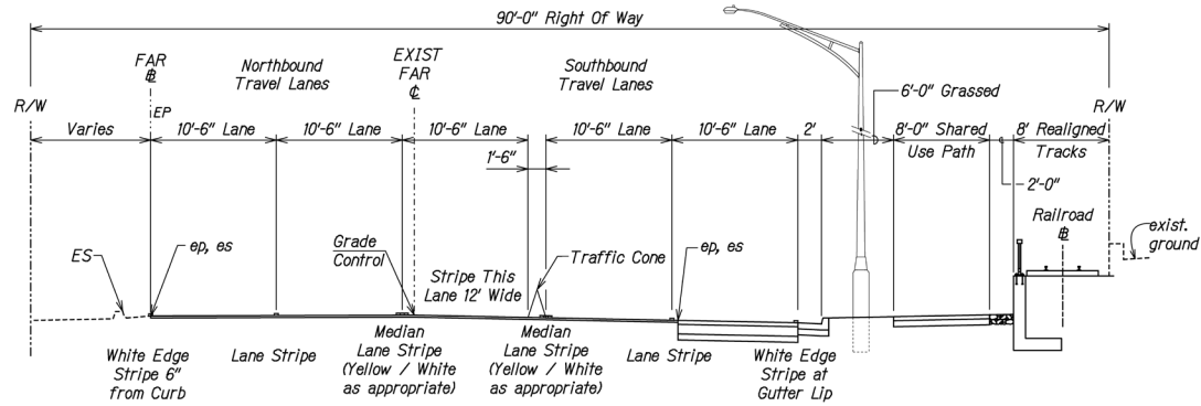
TYPICAL SECTION (INTERIM CONDITION) P.M. Contra-Flow: Helelua St. To Nanakuli Ave. Scale: 1"=5'
