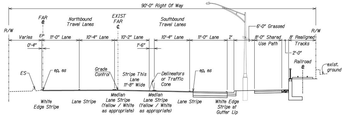
TYPICAL SECTION (FINAL CONDITION) P.M. Contra-Flow: Helelua St. To Nanakuli Ave. Scale: 1"=5'
